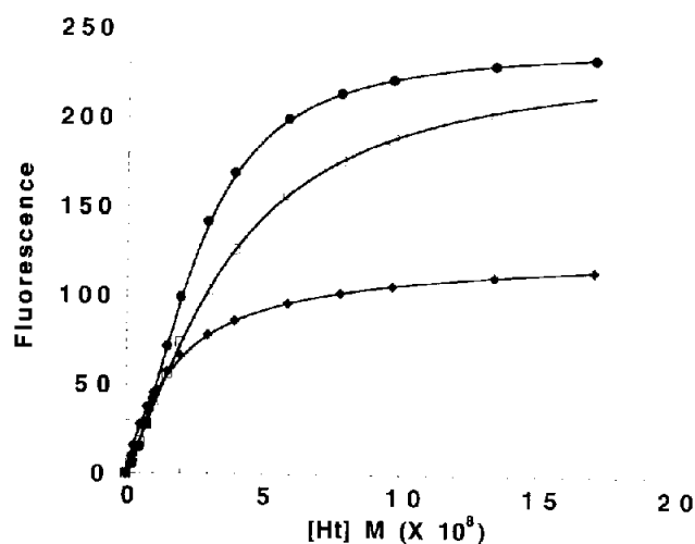
Figure 2. Representative plots of Fluorescence ( F , in arbitrary units) vs total Hoechst 33,258 ( Ht ) concentration at pH 7.0 and 35 °C for 7 at 3.0 \times 10^{-8} M (●), 9.0 \times 10^{-8} M (○) and 18.0 \times 10^{-8} M (◆) in the presence of 1.0 \times 10^{-6} M ctDNA. The theoretical curves which fit the points were computer generated by optimizing the constants in eq 1.
