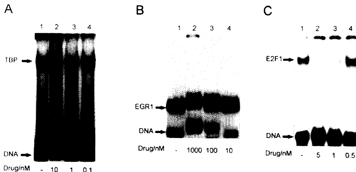
Figure 3. Representative gel mobility shift assay in the presence of 8 . The activity of 8 to inhibit DNA complex formation of transcription factors was demonstrated by gel mobility shift assays. Each of individual transcription factors, TBP (A), EGR1 (B), E2F1 (C), was added to the reaction following treatment with 8 at the indicated concentrations. The upper arrow indicates transcription factor/DNA complex and the lower arrow indicates free DNA.
