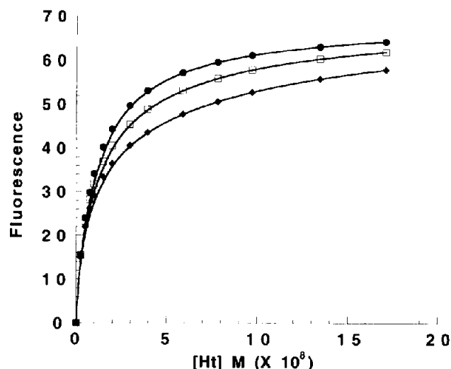
Figure 1. Representative plots of fluorescence ( F , in arbitrary units) vs total Hoechst 33,258 ( Ht ) concentration at pH 7.0 and 35 °C for 7 at 5.0 \times 10^{-6} M (●), 7.5 \times 10^{-6} M (□) and 1.0 \times 10^{-6} M (◆) in the presence of 5.0 \times 10^{-9} M d(\text{GGCGCA}_3\text{T}_3\text{GGCGG})/d(\text{CCGCCA}_3\text{T}_3\text{GCGCC}) . The theoretical curves which fit the points were computer generated by optimizing the constants in eq 1.
